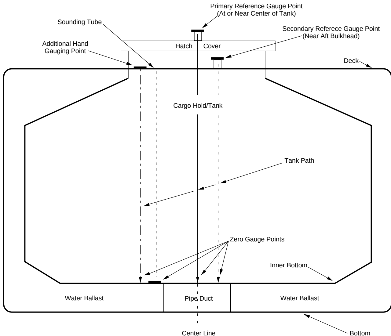
Figure 5—Transverse Section Through Cargo Hold/Tank of a Combination Carrier (OBO) Showing Recommended Gauge Point Locations
