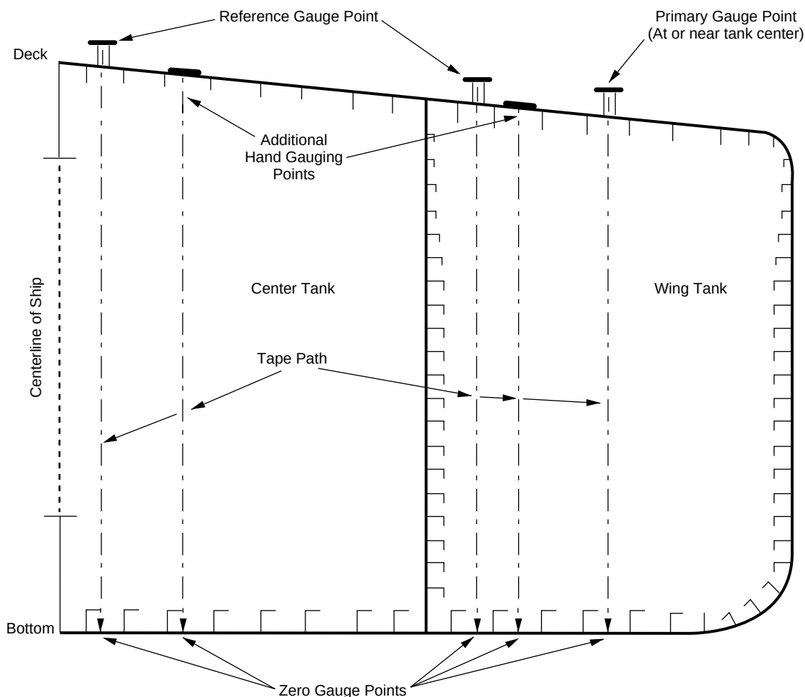
Figure 3—Transverse Section Through Typical Cargo Tank Showing Recommended Gauge Point Locations for Tankers
