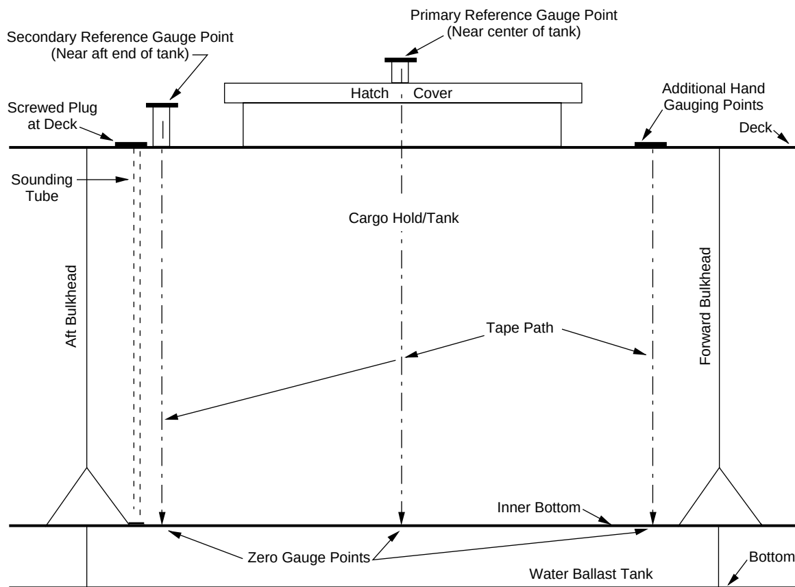
Figure 4—Longitudinal Section Through Cargo Hold/Tank of a Combination Carrier (OBO) Showing Recommended Gauge Point Locations
